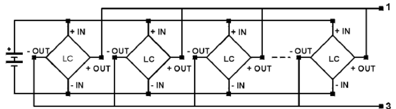
4 OR MORE CELLS CONNECTED IN PARALLEL
