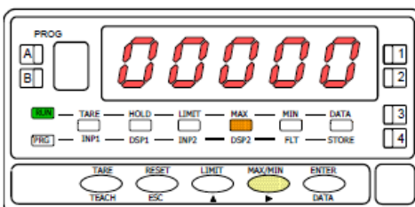
[73.6] Reset of the peak memory
