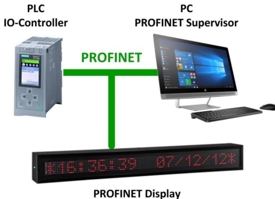
Fig. 1 Profinet communication
