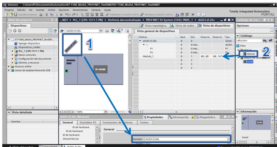
Fig. 12 Assign the E/S addresses of the devices.
